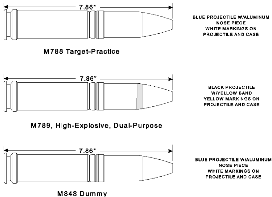
Figure 5-4. 30mm munitions
