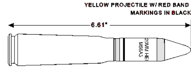
M56A3/A4 High-Explosive Incendiary
