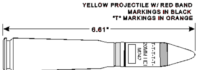
M242, M242A1 High-Explosive Incendiary
