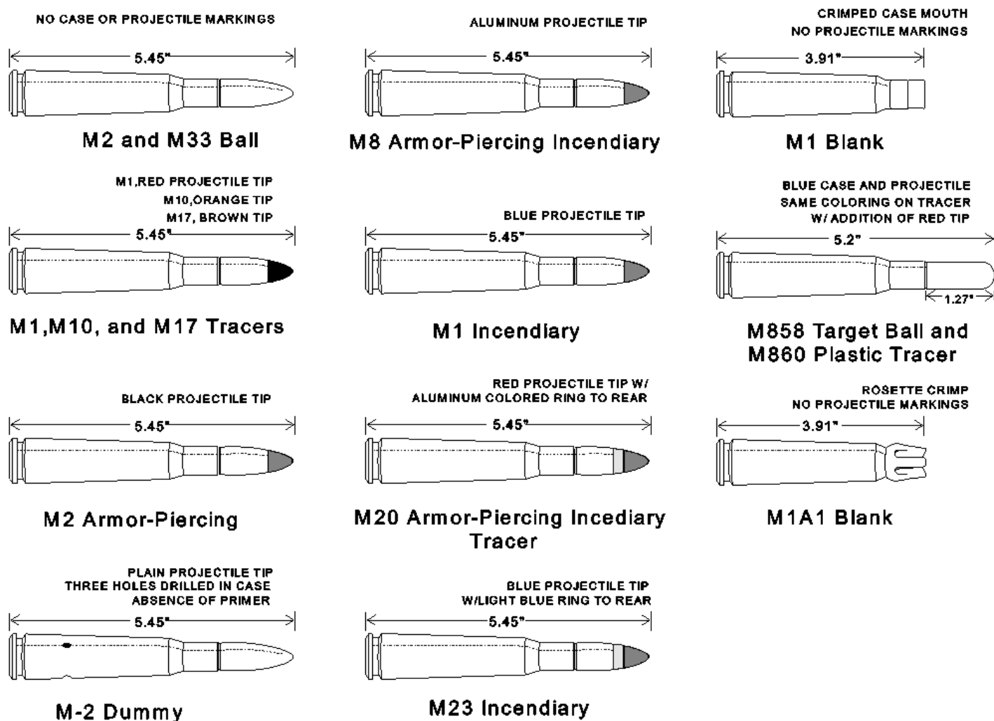
Figure 5-2. .50-caliber munitions
