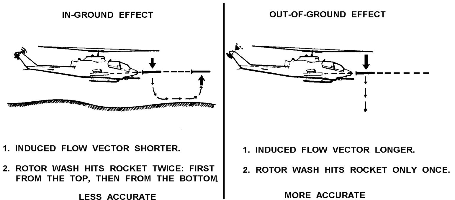
Figure 4-2. Rotor downwash error
