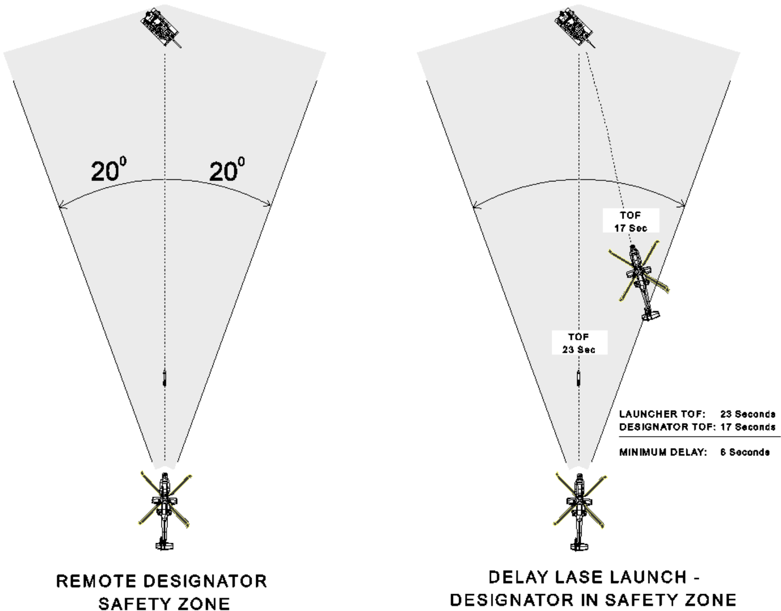
Figure 5-13. Designator avoidance area
