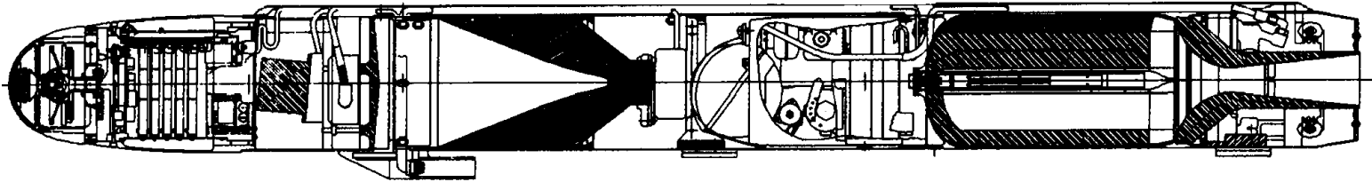
Figure 5-9. Hellfire profile
