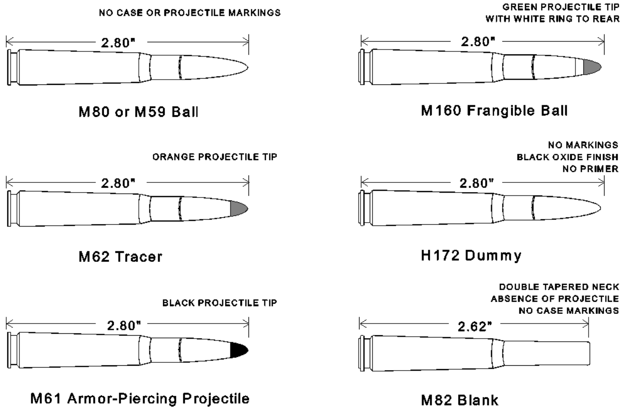
Figure 5-1. 7.62mm munitions
